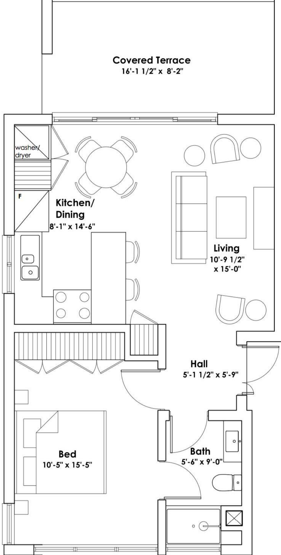
Unit Type A: 1 Bedroom End Unit Ground Floor Plan
